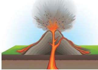
Volcano cross-section.
